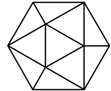
Icosahedron
